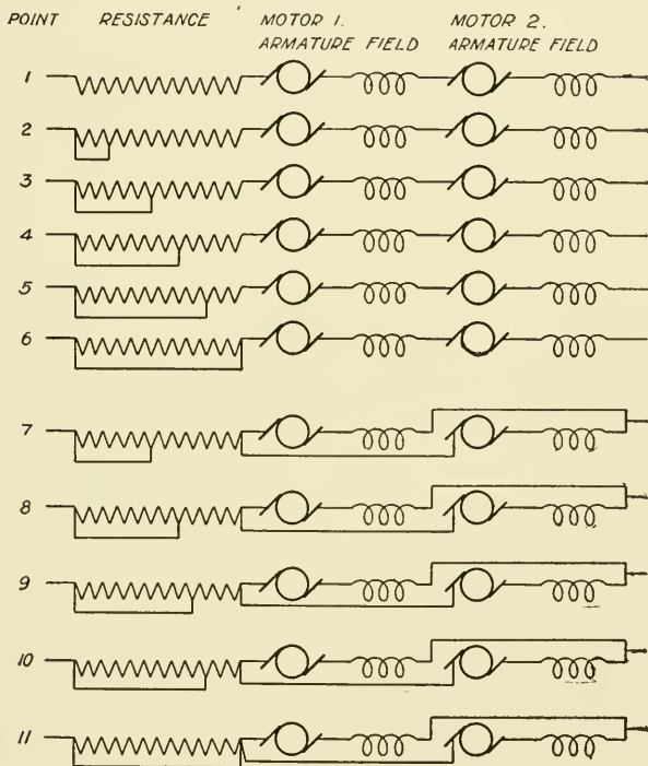
Fig. 48. Controller Diagram
